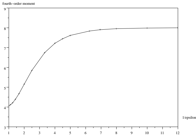
Figure 1. Evolution in 1/\varepsilon of the fourth-order moment of the Boltzmann equation.
