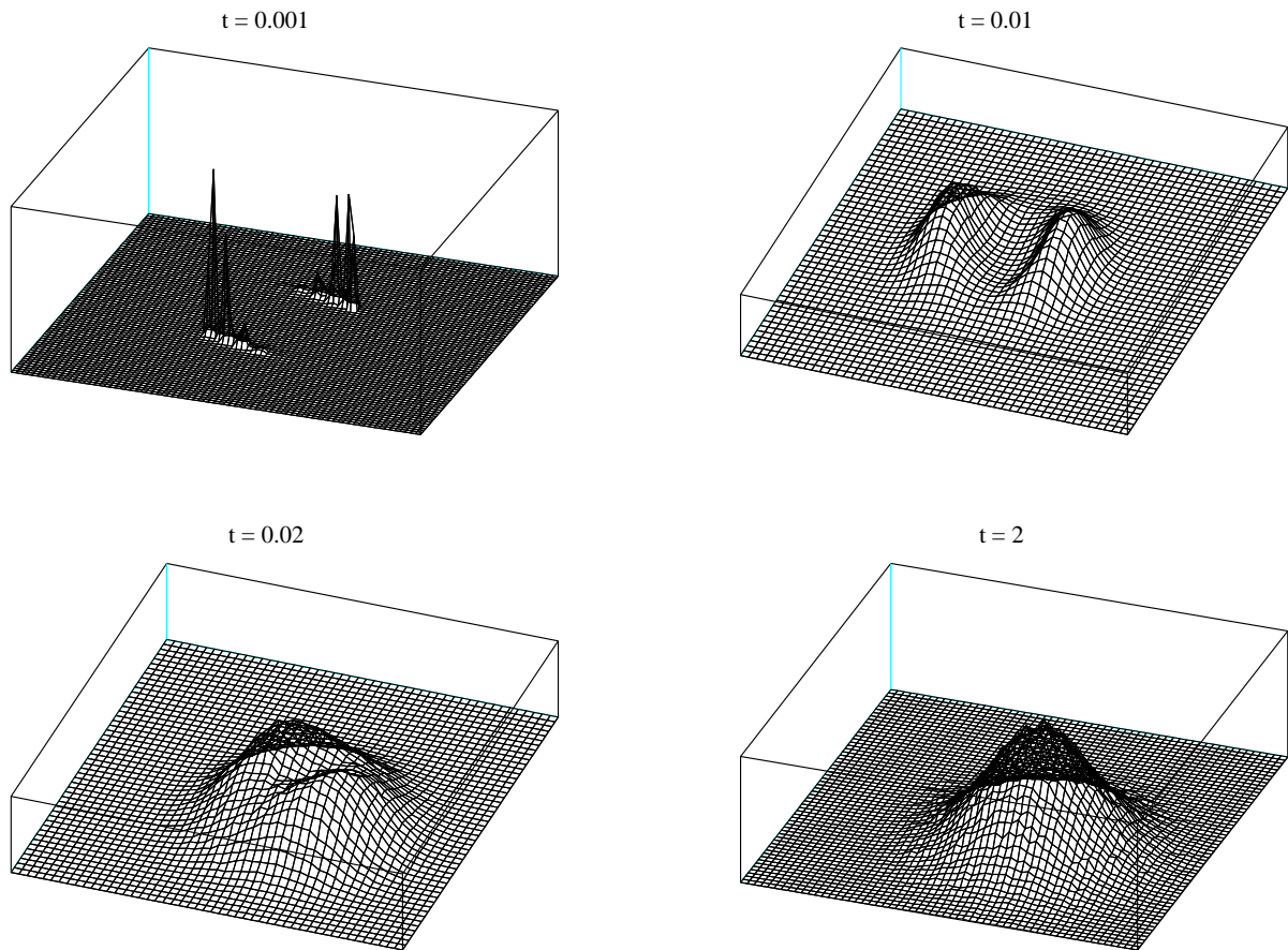
Figure 2. Evolution in time of the solution of the Landau equation.
