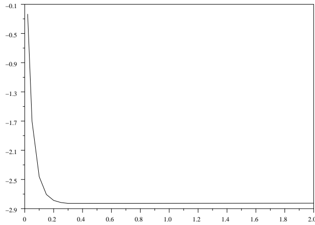
Figure 3. Evolution in time of the entropy.
